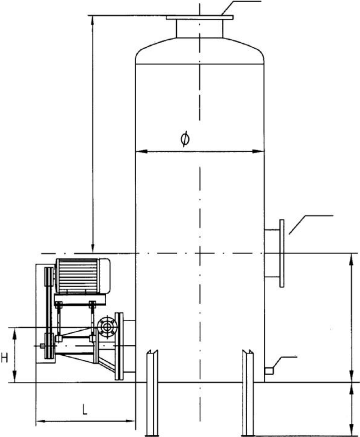
Pre-Separator complete with Liq-Evac pump, Typical Layout
